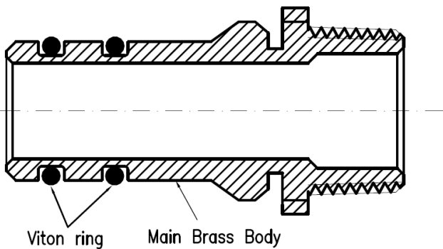
Collector Inlet / outlet adapter to 3/4" NPT
