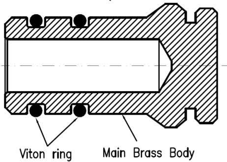
End cup
